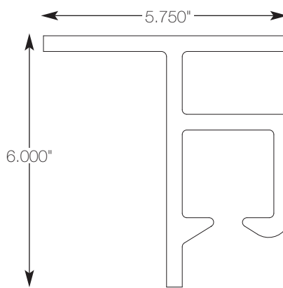
ALUMINUM T-TRACK
