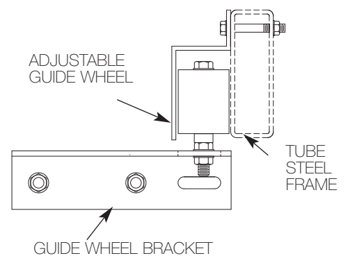
GUIDE WHEEL
