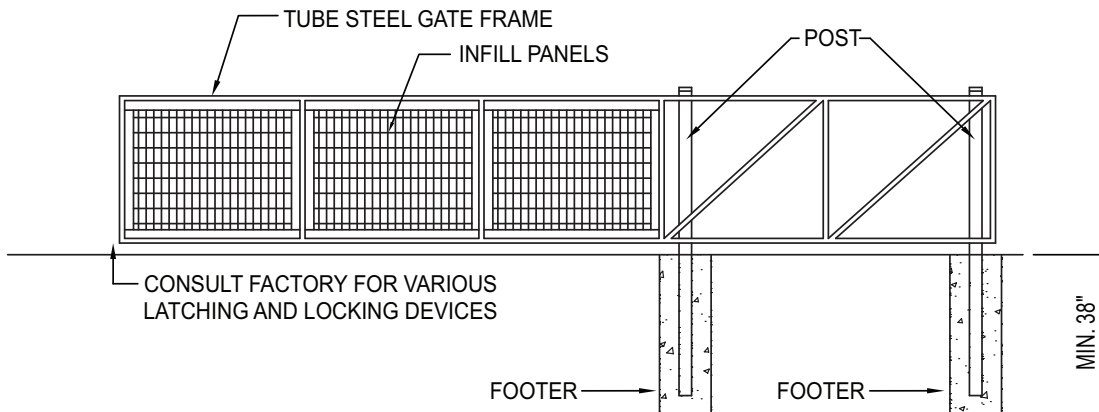
ELEVATION VIEW
